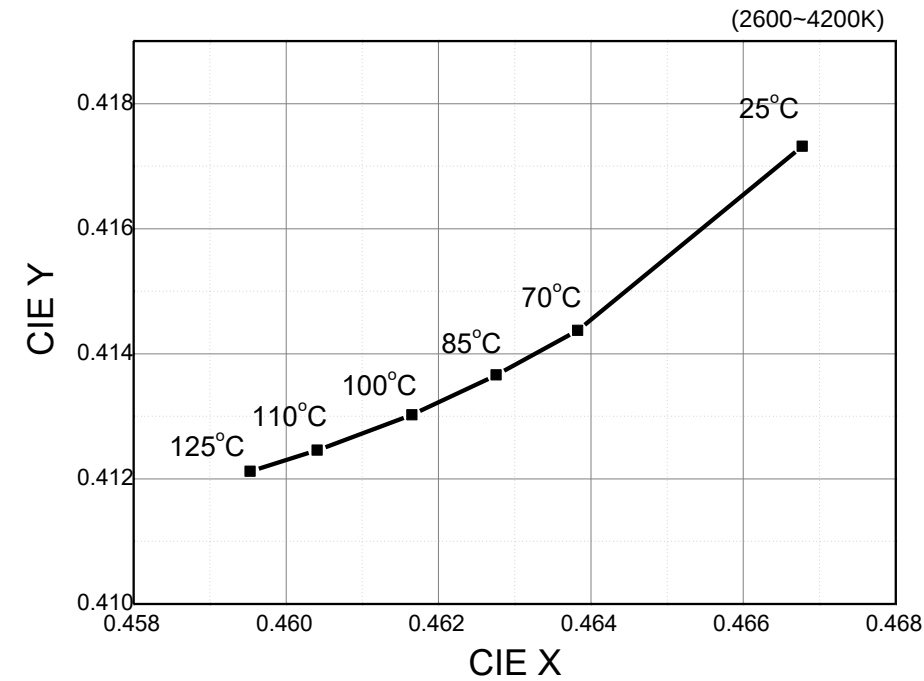
Fig 8. Chromaticity Coordinate vs. Junction Temperature, I_F=150\text{mA}
