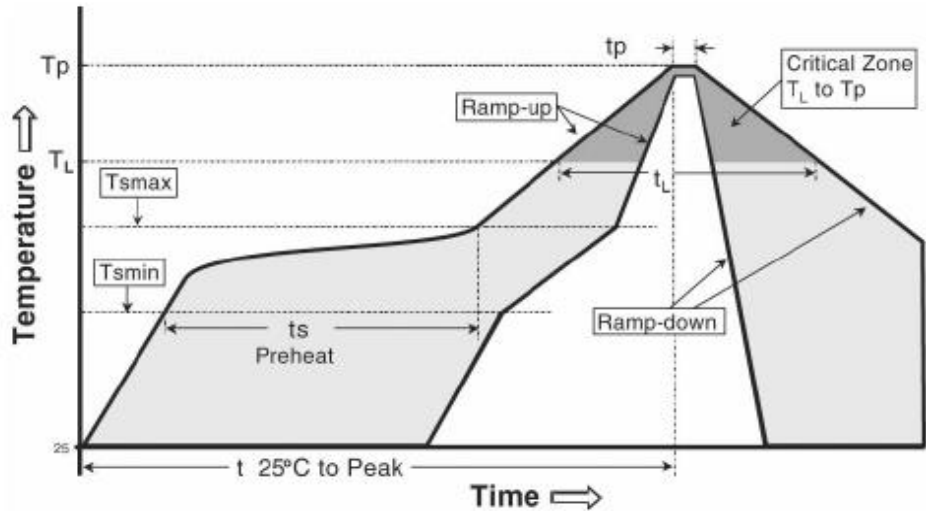
IPC/JEDEC J-STD-020
